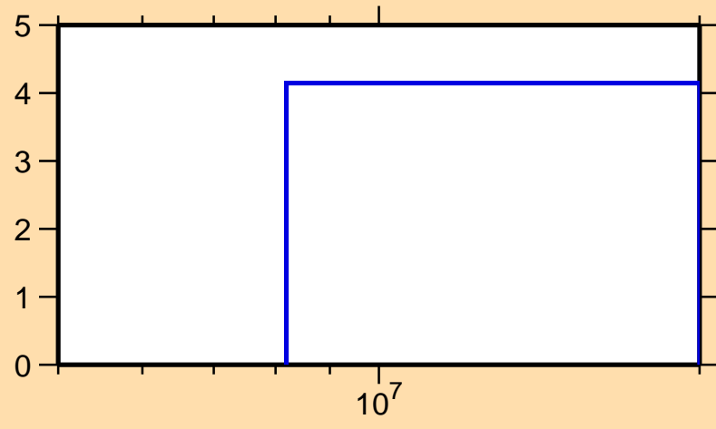
\Delta\sigma/\sigma vs. E for 255
