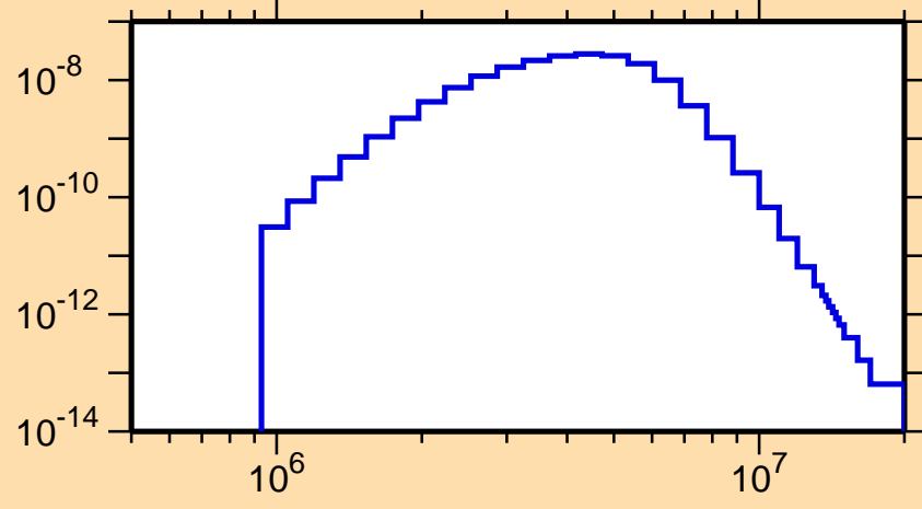
\sigma vs. E for ^{258}_{3} )
