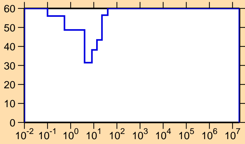
\Delta\sigma/\sigma vs. E for ^{258}\text{Po}
