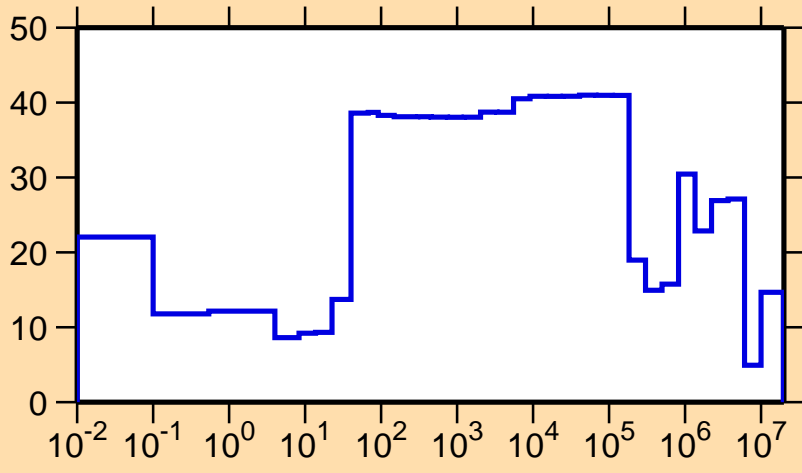
\Delta\sigma/\sigma vs. E for ^{258}\text{Ge}
