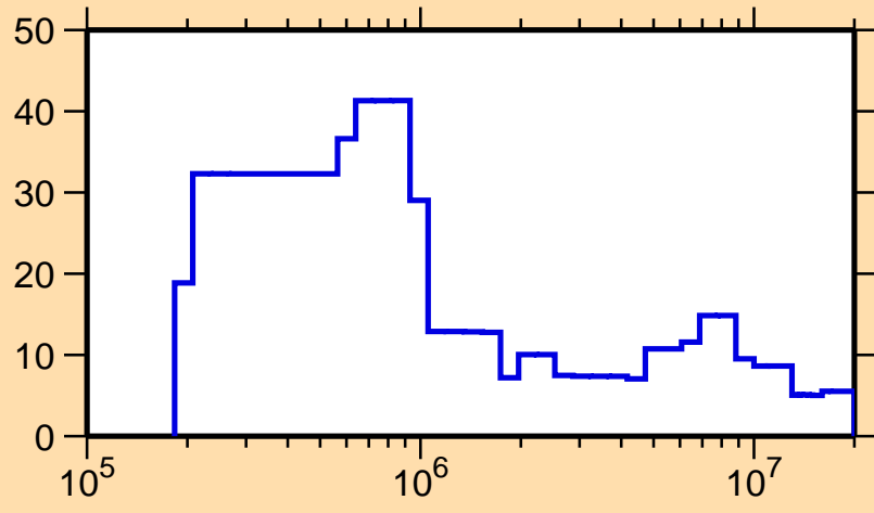
\Delta\sigma/\sigma vs. E for ^{260}\text{Po}
