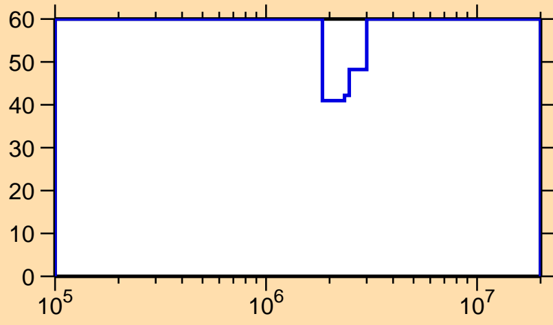
\Delta\sigma/\sigma vs. E for ^{261}_{1}\text{Pb}
