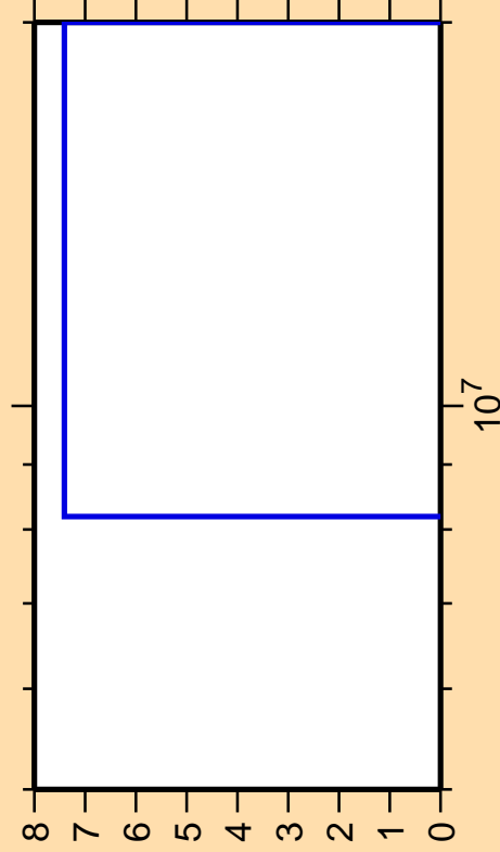
\Delta\sigma/\sigma vs. E for ^{263}
