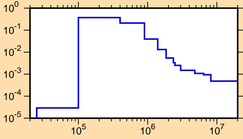
\sigma vs. E for ^{265}\text{Po}
