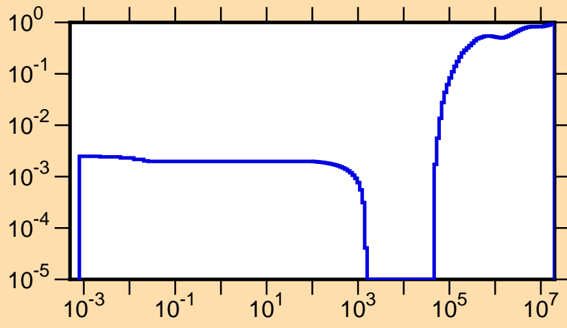
\mu vs. E for ^{267}
