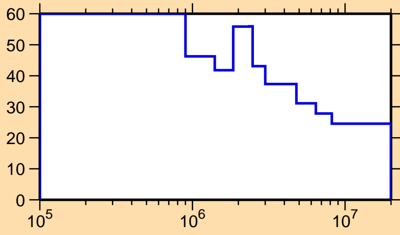
\Delta\sigma/\sigma vs. E for ^{280}\text{Po}
