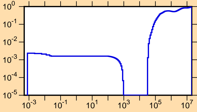
\mu vs. E for ^{281}
