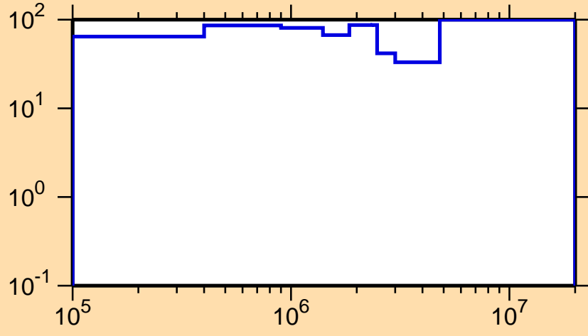
\Delta\sigma/\sigma vs. E for ^{281}\text{P}
