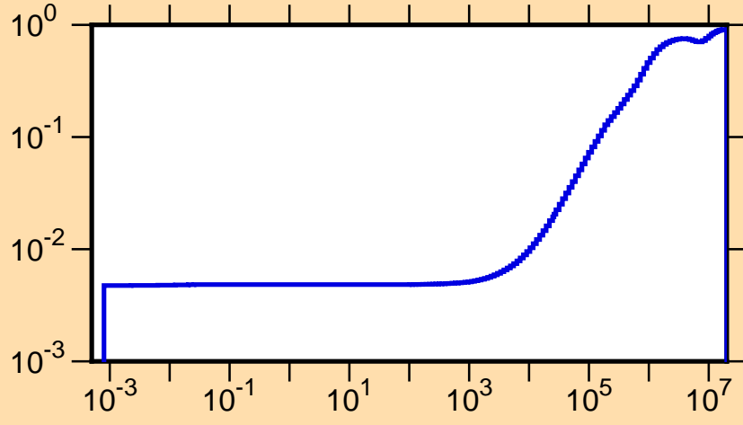
\mu vs. E for ^{142}\text{Dy}(\text{mt251})
