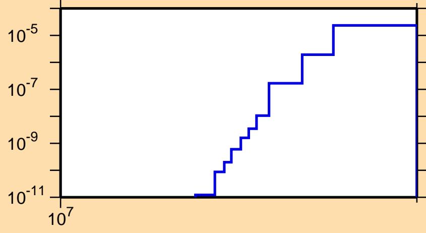
\sigma vs. E for ^{142}\text{Dy}(n,\text{pt})
