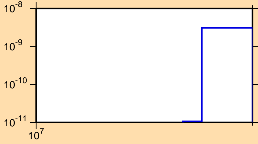
\sigma vs. E for ^{142}\text{Dy}(n,nd)
