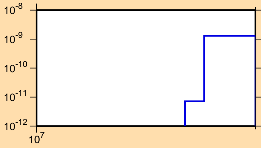
\sigma vs. E for ^{142}\text{Dy}(n,2n\alpha)
