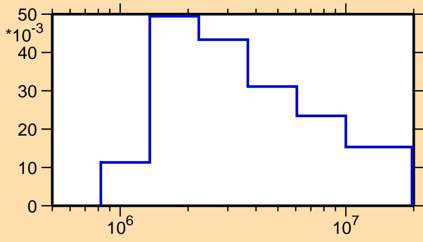
\sigma vs. E for ^{142}\text{Dy}(n,n_2)
