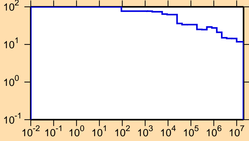
\Delta\sigma/\sigma vs. E for ^{142}\text{Dy}(n,\text{nonel.})
