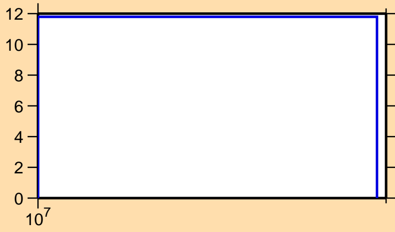
\Delta\sigma/\sigma vs. E for ^{142}\text{Dy}(n,\text{nonel.})
