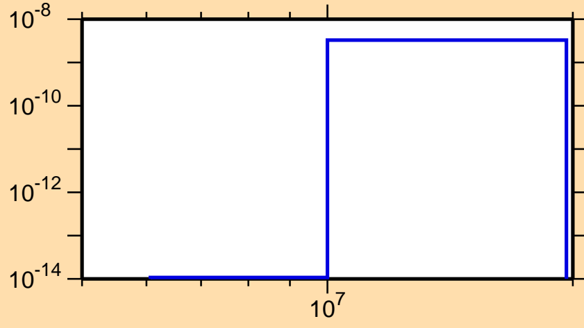
\sigma vs. E for ^{142}\text{Dy}(\text{mt117})
