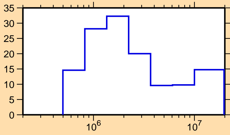
\Delta\sigma/\sigma vs. E for ^{142}\text{Dy}(n,\text{tot.})
