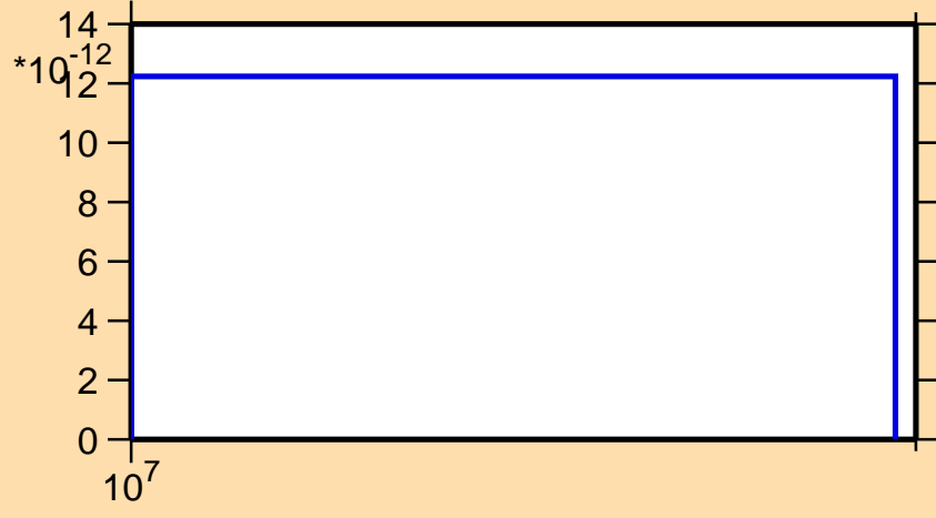
\sigma vs. E for ^{142}\text{Dy} (mt 34)
