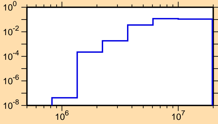
\sigma vs. E for ^{142}\text{Dy}(n,n\text{cont.})
