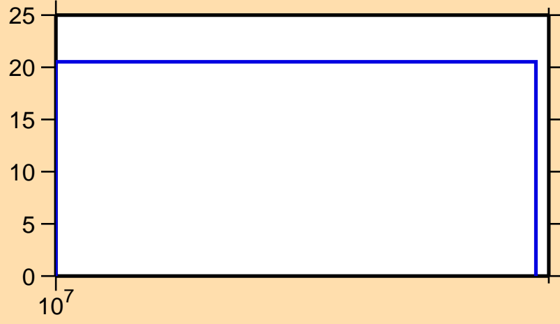
\Delta\sigma/\sigma vs. E for ^{142}\text{Dy}(n,\text{el.})
