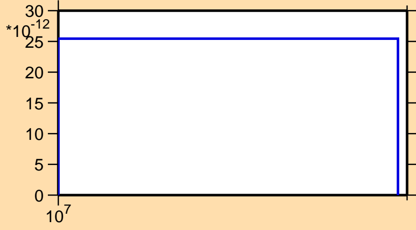
\sigma vs. E for ^{142}\text{Dy}(n,\text{nd})
