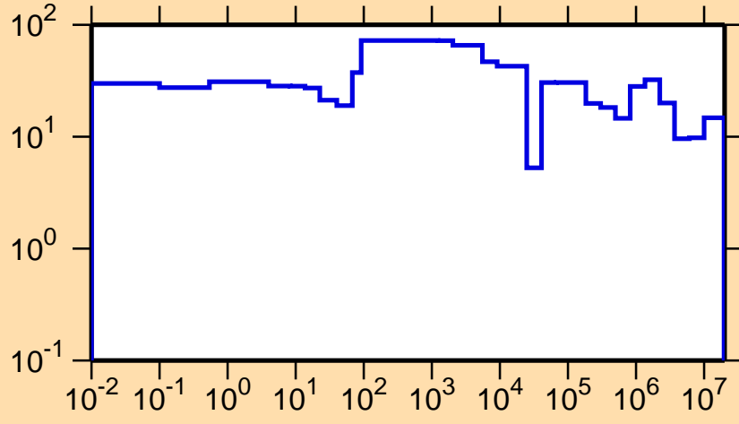
\Delta\sigma/\sigma vs. E for ^{142}\text{Dy}(n,\text{tot.})
