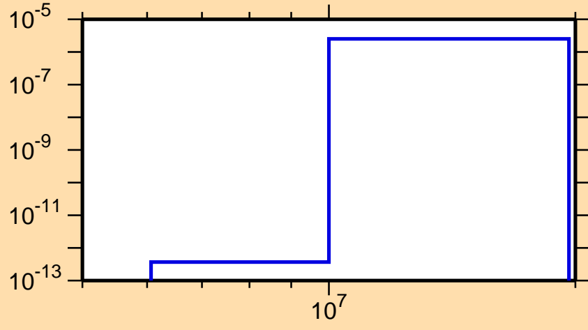
\sigma vs. E for ^{142}\text{Dy} (mt 45)
