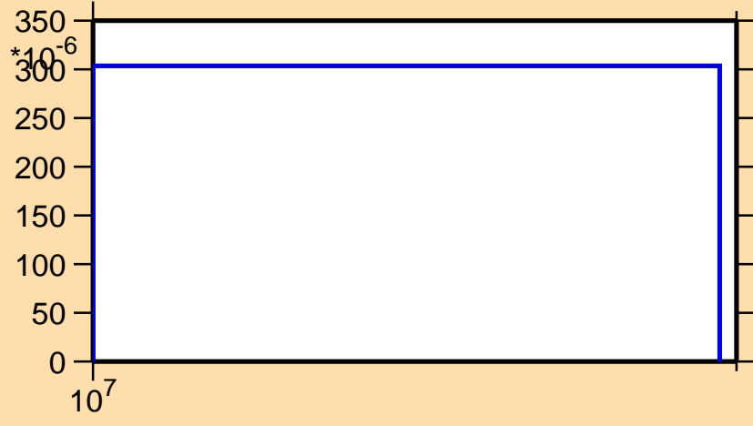
\sigma vs. E for ^{142}\text{Dy}(n,2n)
