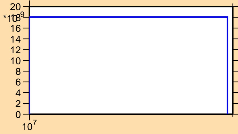
\sigma vs. E for ^{142}\text{Dy}(n,2np)
