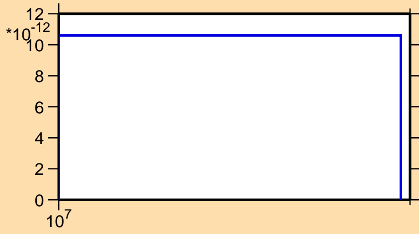
\sigma vs. E for ^{142}\text{Dy}(n,2n\alpha)
