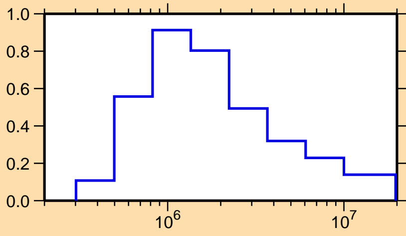
\sigma vs. E for ^{142}\text{Dy}(n,n_1)
