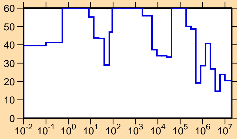
\Delta\sigma/\sigma vs. E for ^{142}\text{Dy}(n,\text{el.})
