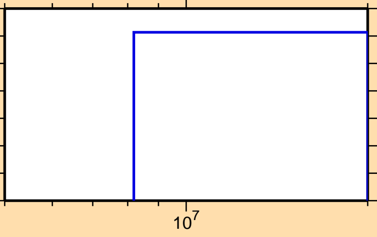
\sigma vs. E for ^{142}\text{Dy}(n,t)
