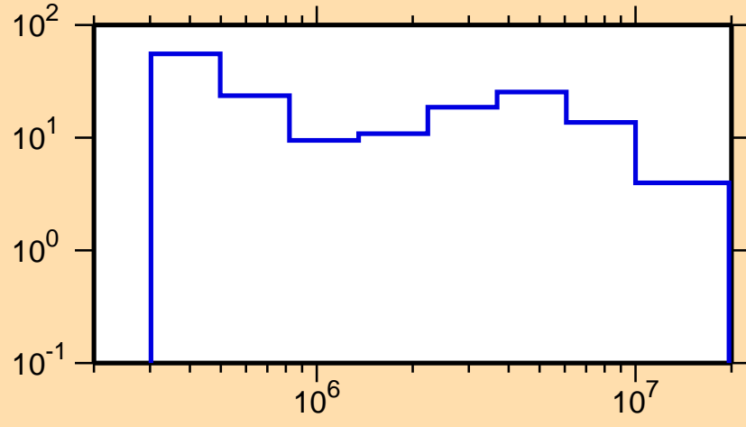
\Delta\sigma/\sigma vs. E for ^{143}\text{Dy}(n,el.)
