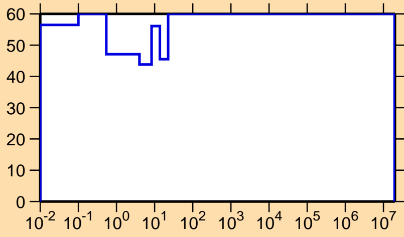
\Delta\sigma/\sigma vs. E for ^{143}\text{Dy}(n,\gamma)
