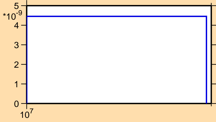
\sigma vs. E for ^{143}\text{Dy}(n,\text{nd})
