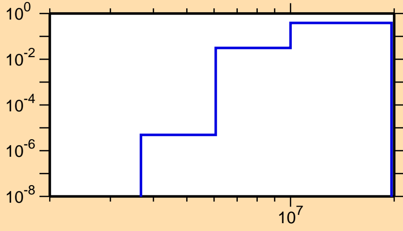
\sigma vs. E for ^{143}\text{Dy}(n,np)
