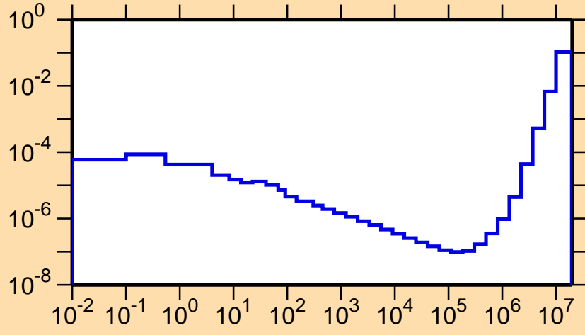
\sigma vs. E for ^{143}\text{Dy}(n,p\alpha)
