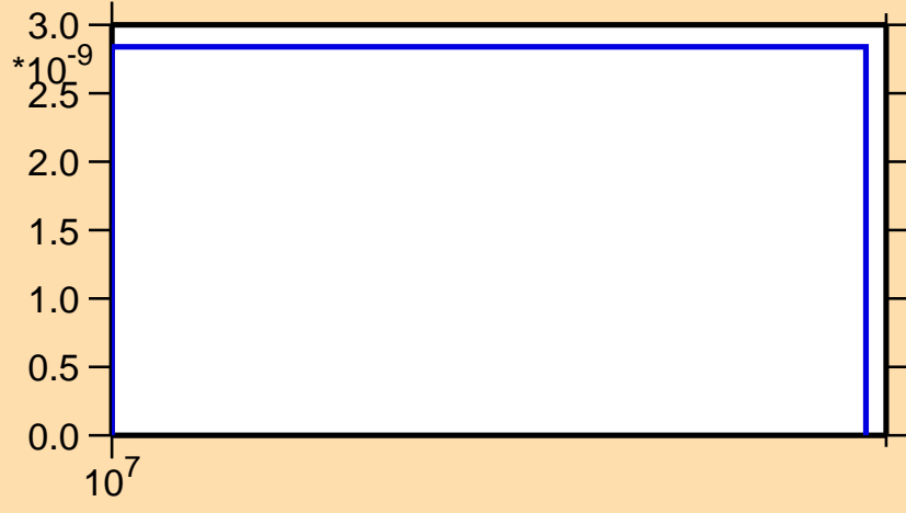
\sigma vs. E for ^{143}\text{Dy} (mt 34)
