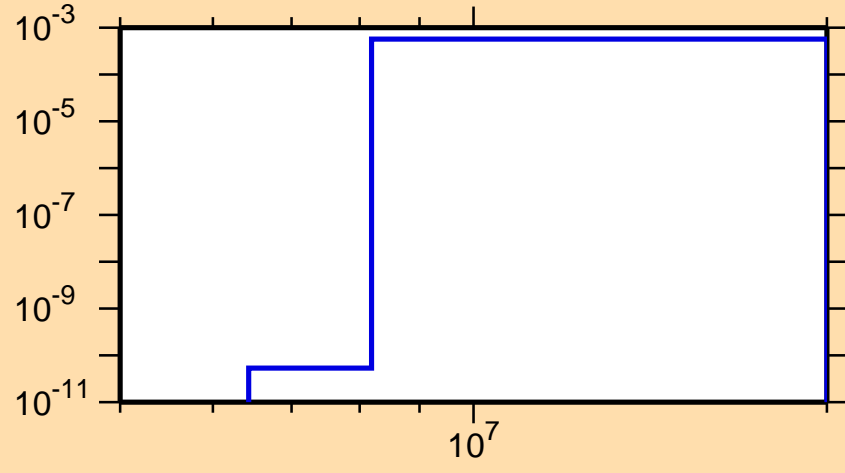
\sigma vs. E for ^{143}\text{Dy}(n,\text{pd})
