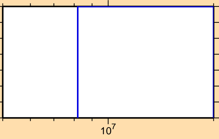
\sigma vs. E for ^{143}\text{Dy}(n,\text{pt})
