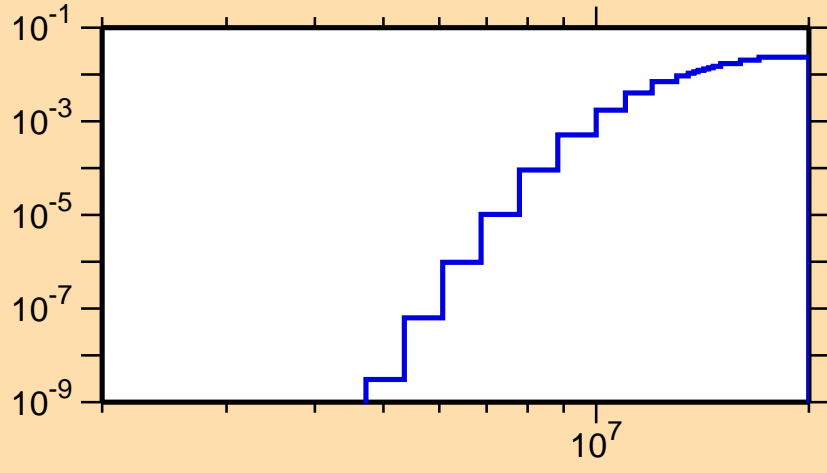
\sigma vs. E for ^{145}\text{Dy}(n,d)
