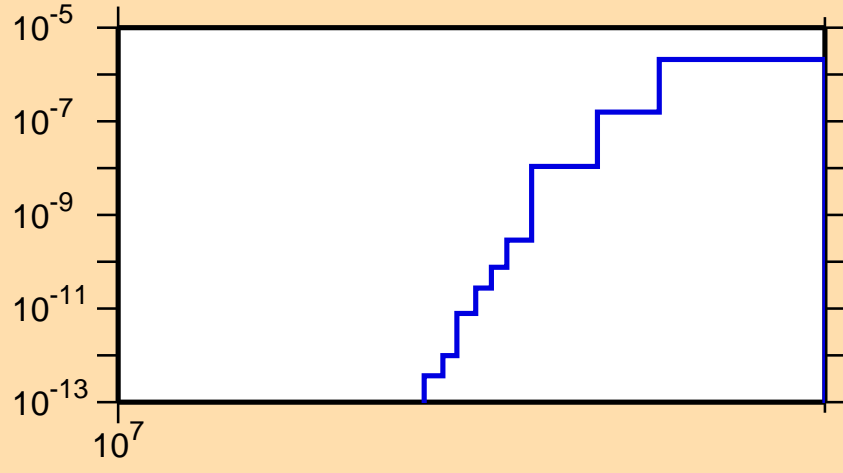
\sigma vs. E for ^{145}\text{Dy}(n,nd)
