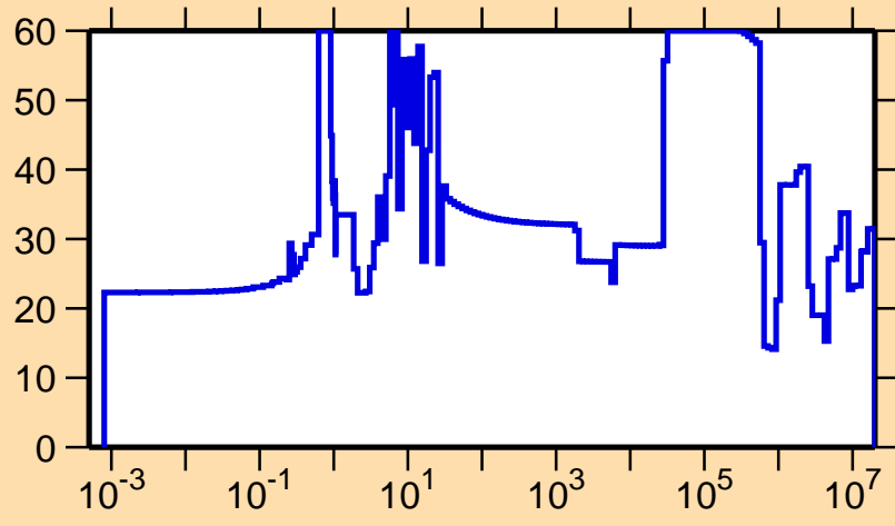
\Delta\sigma/\sigma vs. E for ^{145}\text{Dy}(n,\text{el.})
