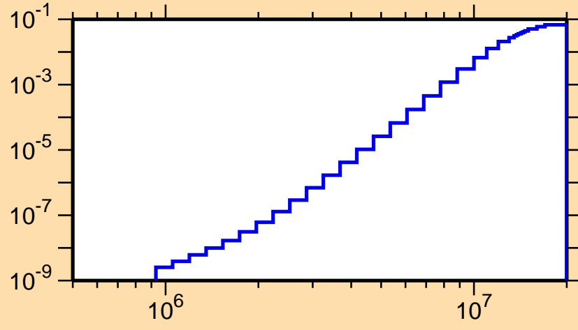
\sigma vs. E for ^{145}\text{Dy}(n,p\alpha)
