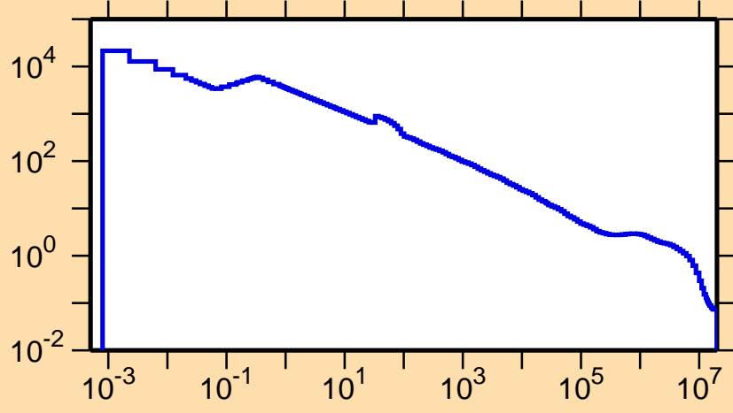
\sigma vs. E for ^{145}\text{Dy}(n,p)
