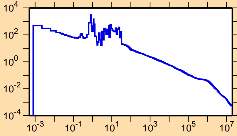
\sigma vs. E for ^{145}\text{Dy}(n,\gamma)
