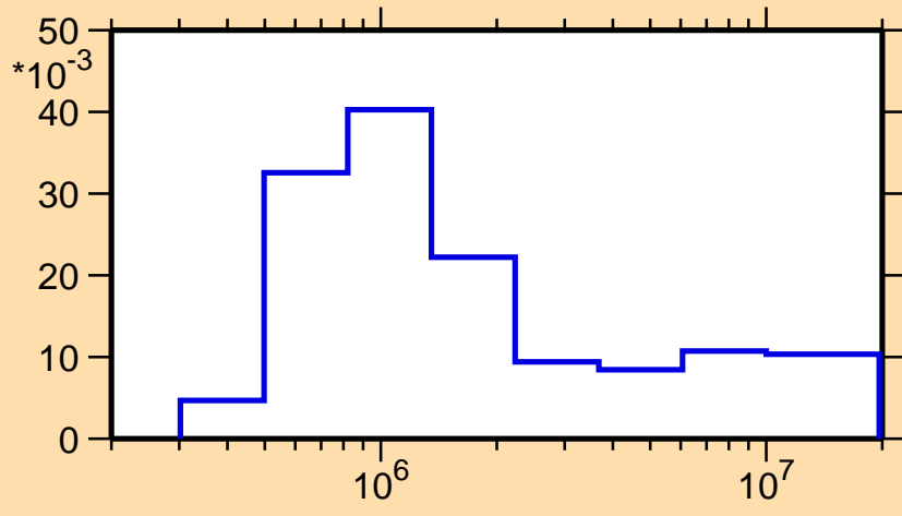
\sigma vs. E for ^{145}\text{Dy}(n,n_3)
