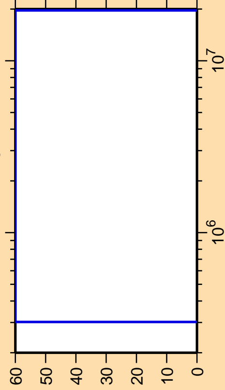
\Delta\sigma/\sigma vs. E for ^{145}\text{Dy}(n,n_3)
