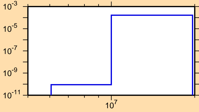
\sigma vs. E for ^{145}\text{Dy}(n,\text{pd})
