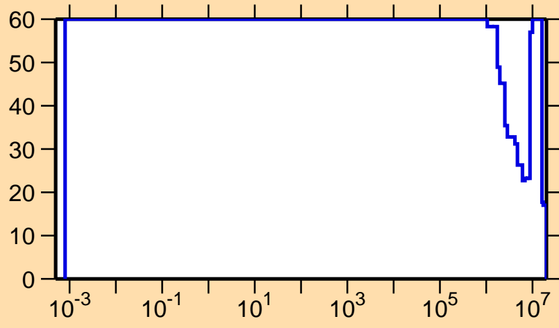
\Delta\sigma/\sigma vs. E for ^{145}\text{Dy}(n,p)
