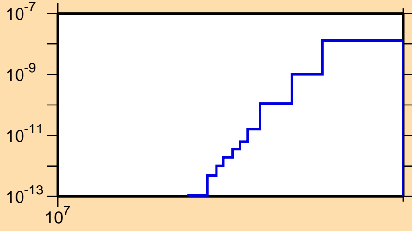
\sigma vs. E for ^{145}\text{Dy} (mt 34)
