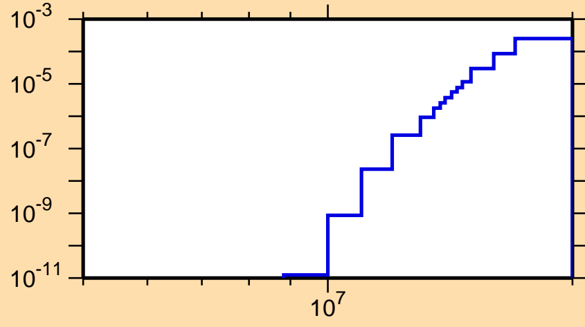
\sigma vs. E for ^{146}\text{Dy}(n,\text{pd})
