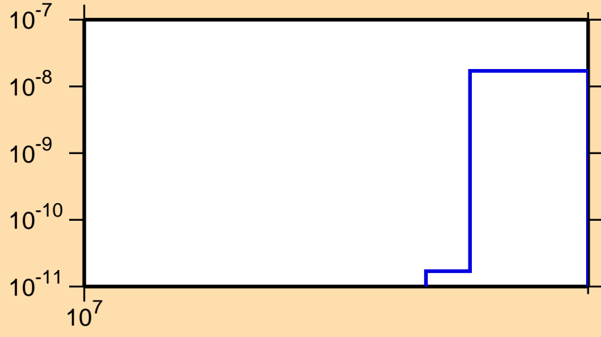
\sigma vs. E for ^{146}\text{Dy}(n,\text{nd})
