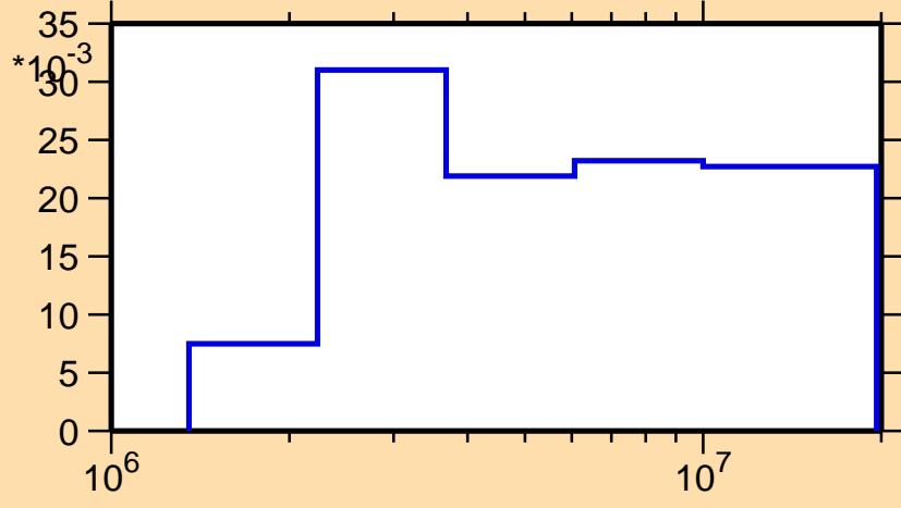
\sigma vs. E for ^{146}\text{Dy}(n,n_3)
