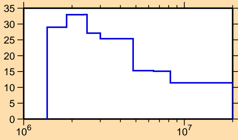
\Delta\sigma/\sigma vs. E for ^{146}\text{Dy}(n,el.)
