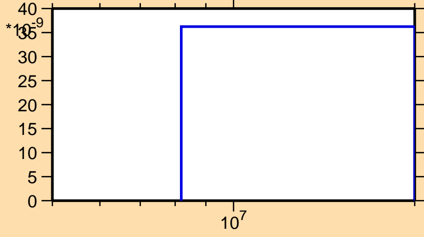
\sigma vs. E for ^{146}\text{Dy} (mt 45)
