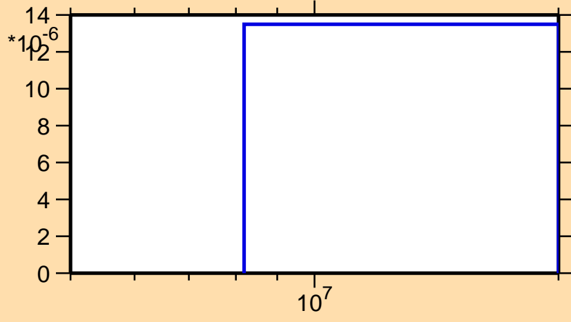
\sigma vs. E for ^{146}\text{Dy}(n,t)
