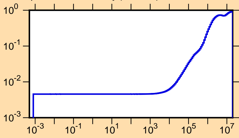
\mu vs. E for ^{148}\text{Dy}(\text{mt251})
