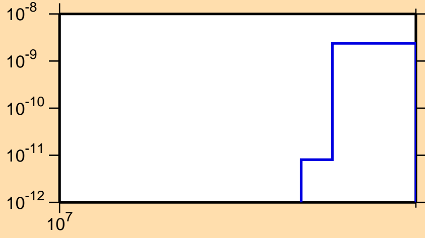
\sigma vs. E for ^{148}\text{Dy}(n,pt)
