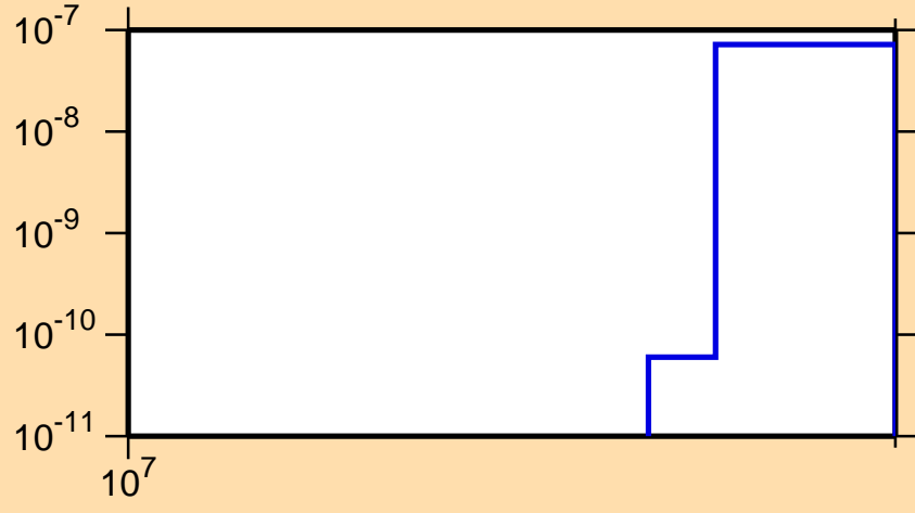
\sigma vs. E for ^{148}\text{Dy}(n,nd)
