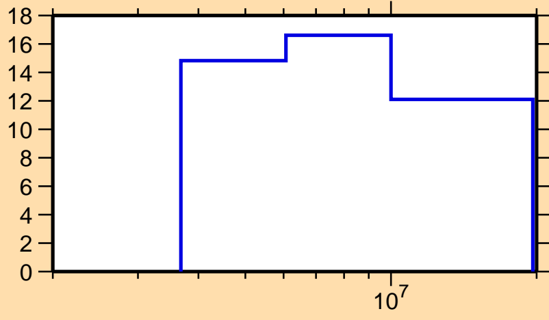
\Delta\sigma/\sigma vs. E for ^{148}\text{Dy}(n,el.)
