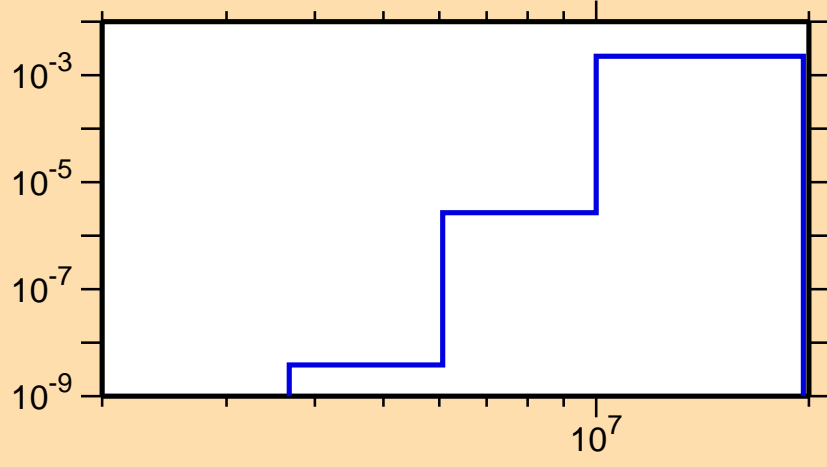
\sigma vs. E for ^{148}\text{Dy}(n,n\alpha)
