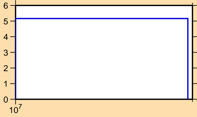
\Delta\sigma/\sigma vs. E for ^{148}\text{Dy}(n,\text{nonel.})
