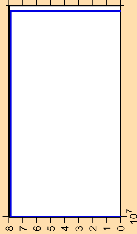
\Delta\sigma/\sigma vs. E for ^{148}\text{Dy}(n,2n\alpha)
