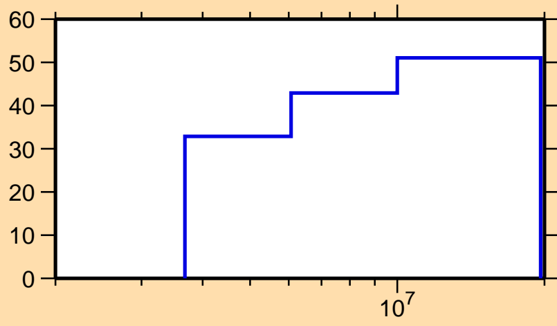
\Delta\sigma/\sigma vs. E for ^{148}\text{Dy}(n,n\text{cont.})
