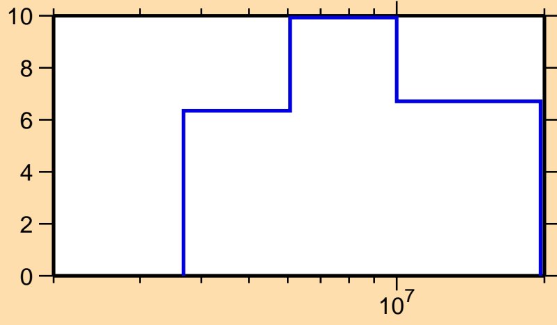
\Delta\sigma/\sigma vs. E for ^{148}\text{Dy}(n, tot.)
