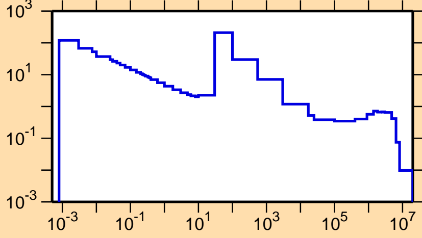
\sigma vs. E for ^{148}\text{Dy}(n,\gamma)
