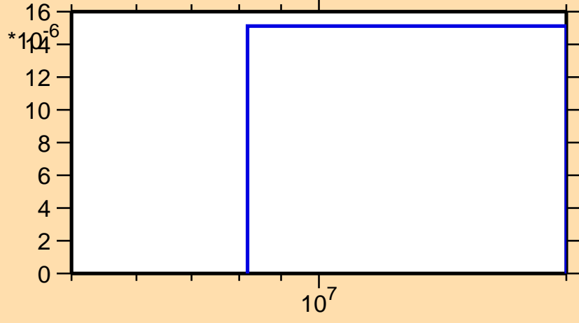
\sigma vs. E for ^{148}\text{Dy}(n,t)
