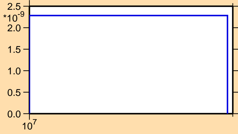
\sigma vs. E for ^{151}\text{Dy}(n,\text{pd})
