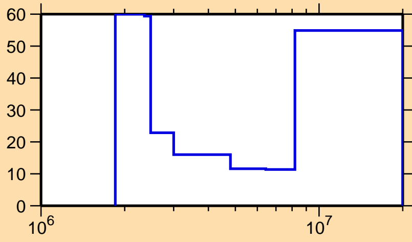
\Delta\sigma/\sigma vs. E for ^{151}\text{Dy}(n,n\text{cont.})
