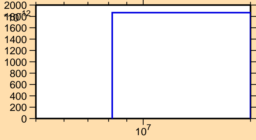
\sigma vs. E for ^{151}\text{Dy}(n,\text{pd})
