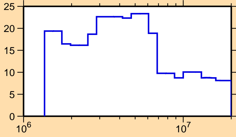
\Delta\sigma/\sigma vs. E for ^{153}\text{Dy}(n,el.)
