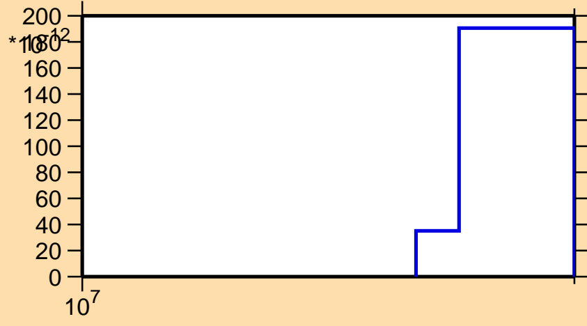
\sigma vs. E for ^{153}\text{Dy}(n,3n\alpha)
