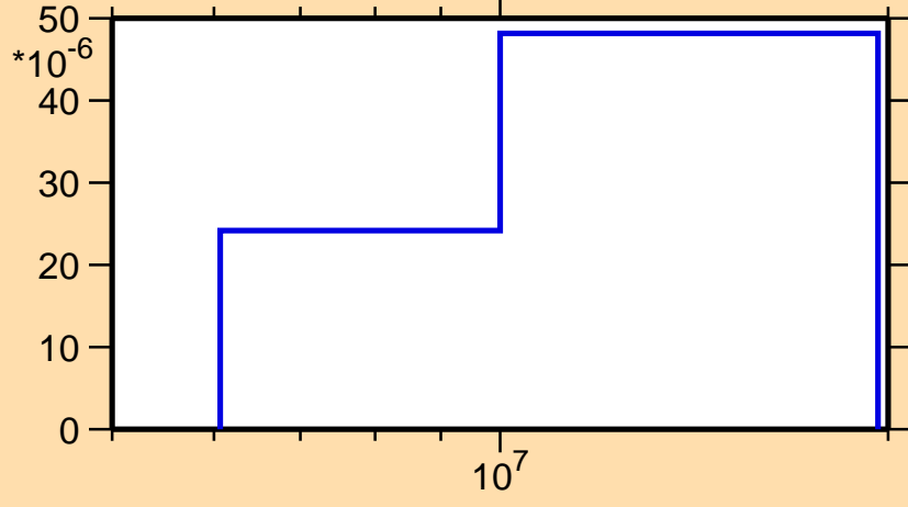
\sigma vs. E for ^{153}\text{Dy}(n,2n\alpha)
