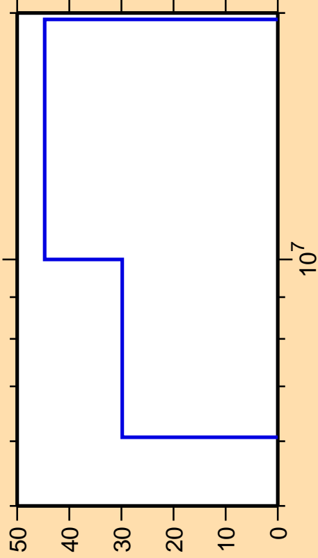
\Delta\sigma/\sigma vs. E for ^{153}\text{Dy}(n,p)
