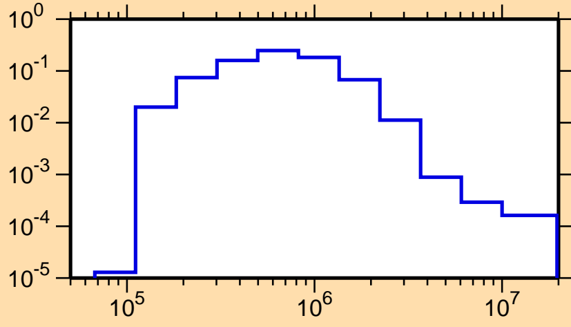
\sigma vs. E for ^{153}\text{Dy}(n,n_1)
