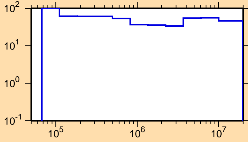
\Delta\sigma/\sigma vs. E for ^{153}\text{Dy}(n,n_1)
