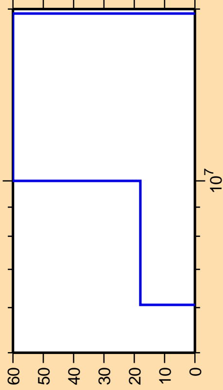
\Delta\sigma/\sigma vs. E for ^{153}\text{Dy}(n,n\text{cont.})
