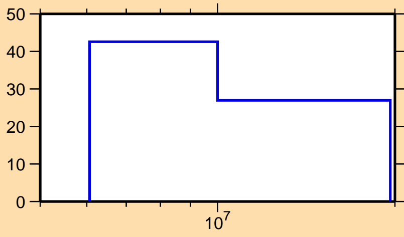
\Delta\sigma/\sigma vs. E for ^{153}\text{Dy}(n,2n)
