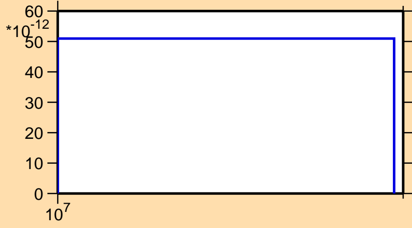
\sigma vs. E for ^{153}\text{Dy} (mt 45)
