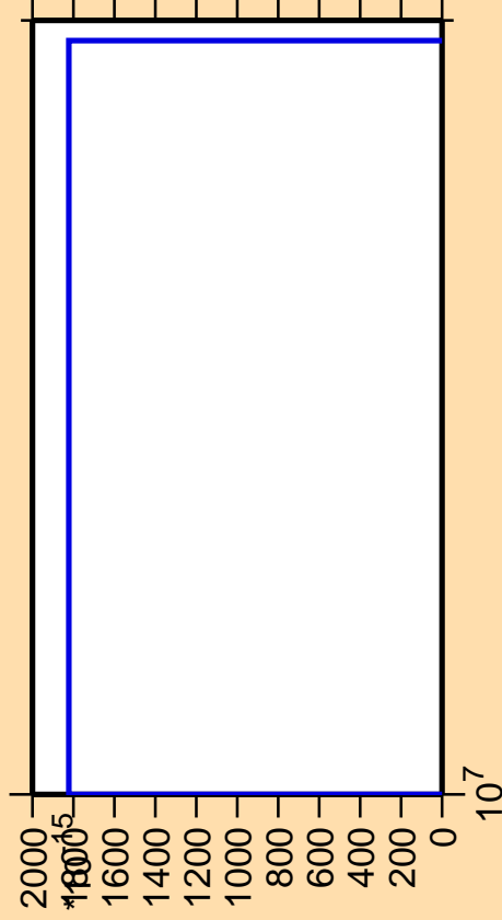
\Delta\sigma/\sigma vs. E for ^{153}\text{Dy} (mt 11)
