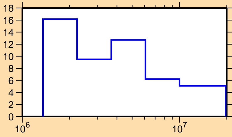
\Delta\sigma/\sigma vs. E for ^{153}\text{Dy}(n,\text{tot.})
