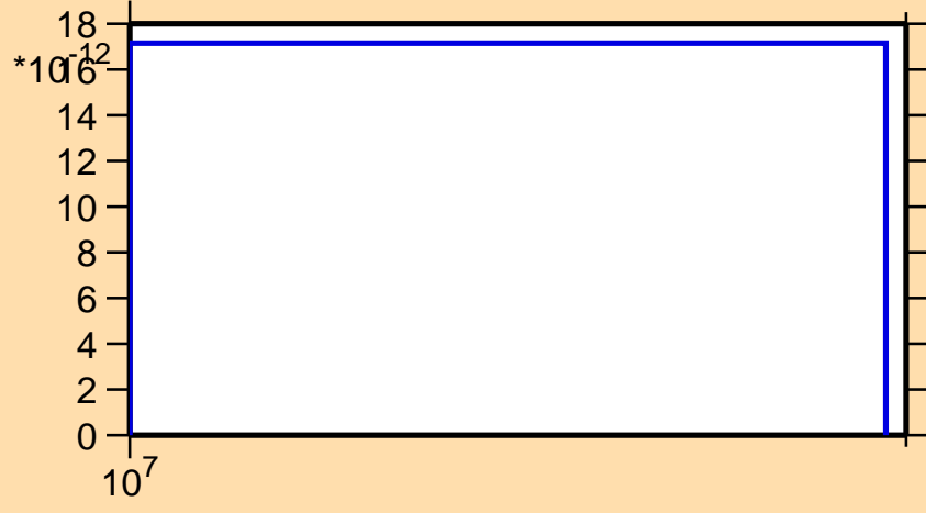
\sigma vs. E for ^{153}\text{Dy}(n,pd)
