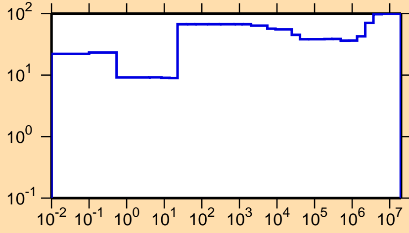
\Delta\sigma/\sigma vs. E for ^{153}\text{Dy}(n,\gamma)
