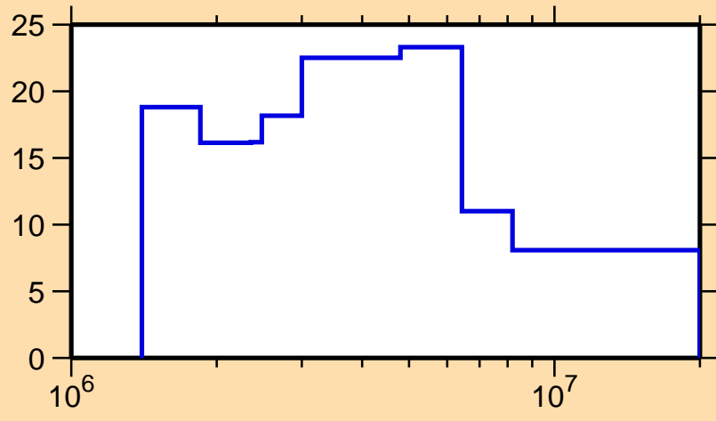
\Delta\sigma/\sigma vs. E for ^{153}\text{Dy}(n,el.)
