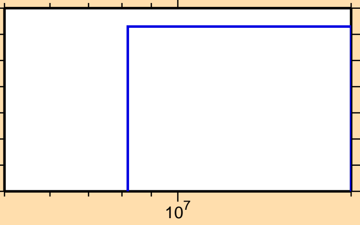
\sigma vs. E for ^{153}\text{Dy}(n,3n\alpha)
