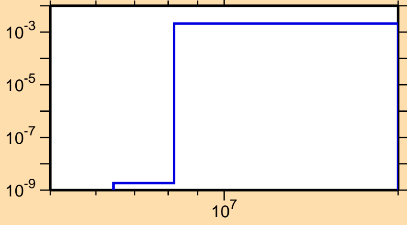
\sigma vs. E for ^{153}\text{Dy}(n,d)
