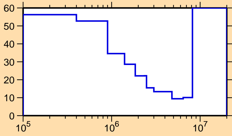
\Delta\sigma/\sigma vs. E for ^{153}\text{Dy}(n,\text{inel.})
