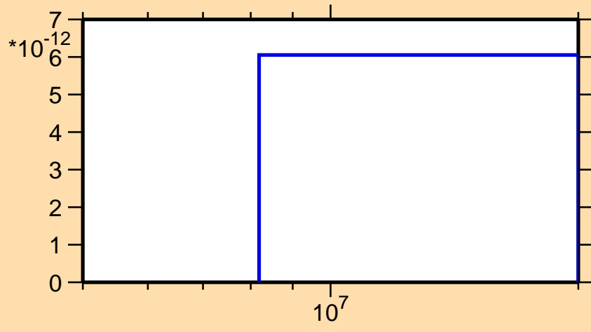
\sigma vs. E for ^{153}\text{Dy}(\text{mt117})
