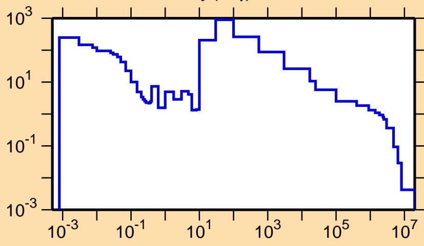
\sigma vs. E for ^{153}\text{Dy}(n,\gamma)
