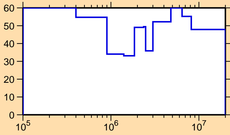
\Delta\sigma/\sigma vs. E for ^{153}\text{Dy}(n,n_1)
