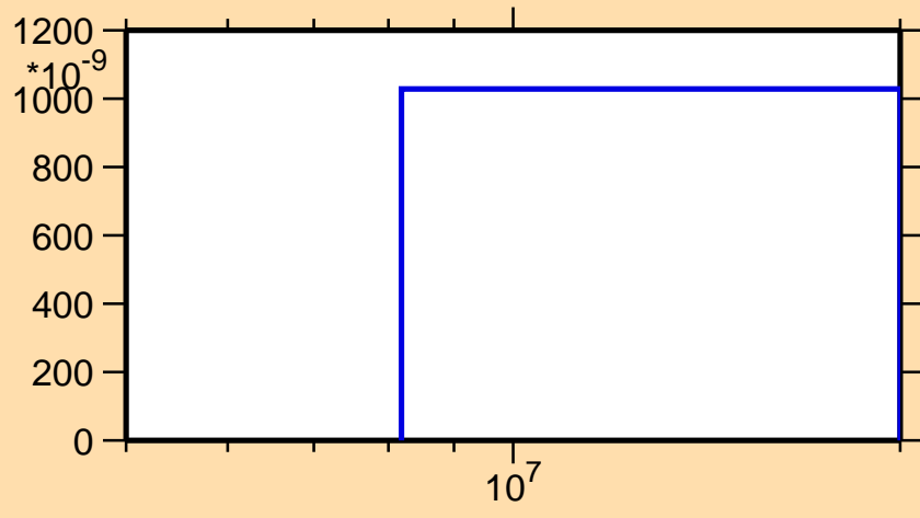
\sigma vs. E for ^{153}\text{Dy}(n,2np)
