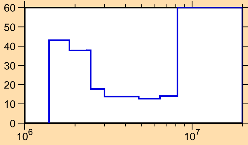
\Delta\sigma/\sigma vs. E for ^{153}\text{Dy}(n,n\text{cont.})
