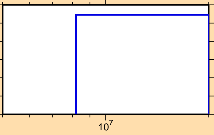
\sigma vs. E for ^{153}\text{Dy}(n,\text{He}3)
