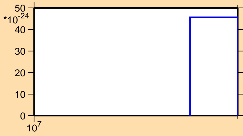
\sigma vs. E for ^{155}\text{Dy} (mt 11)
