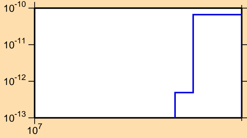
\sigma vs. E for ^{155}\text{Dy}(n,pt)
