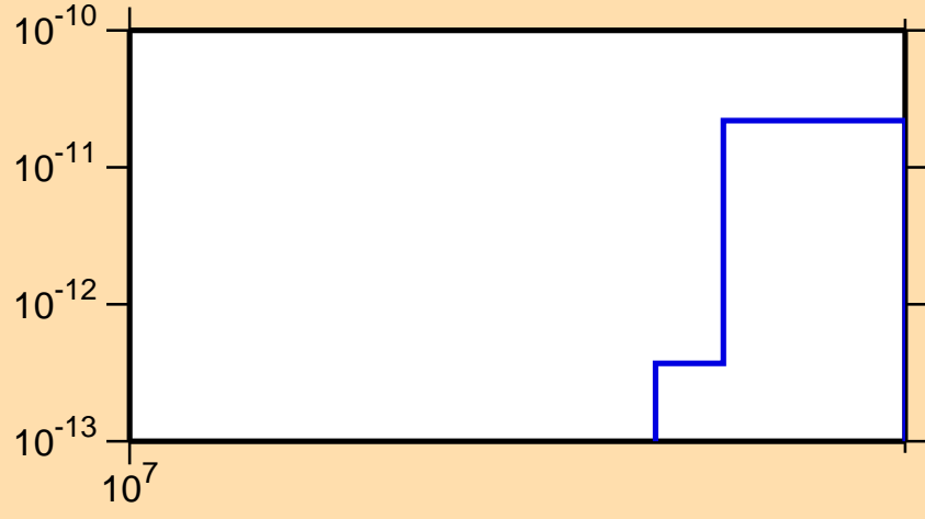
\sigma vs. E for ^{155}\text{Dy}(n,\text{pd})
