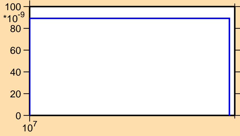
\sigma vs. E for ^{155}\text{Dy}(n,nd)
