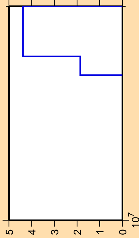
\Delta\sigma/\sigma vs. E for ^{156}\text{Dy}(n,3n\alpha)
