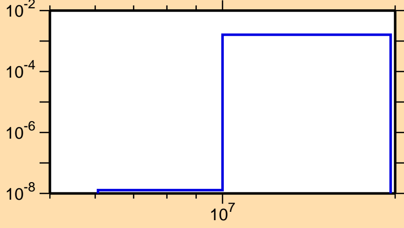
\sigma vs. E for ^{156}\text{Dy}(n,d)
