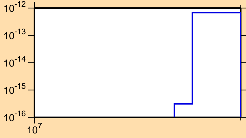
\sigma vs. E for ^{157}\text{Dy} (mt 34)
