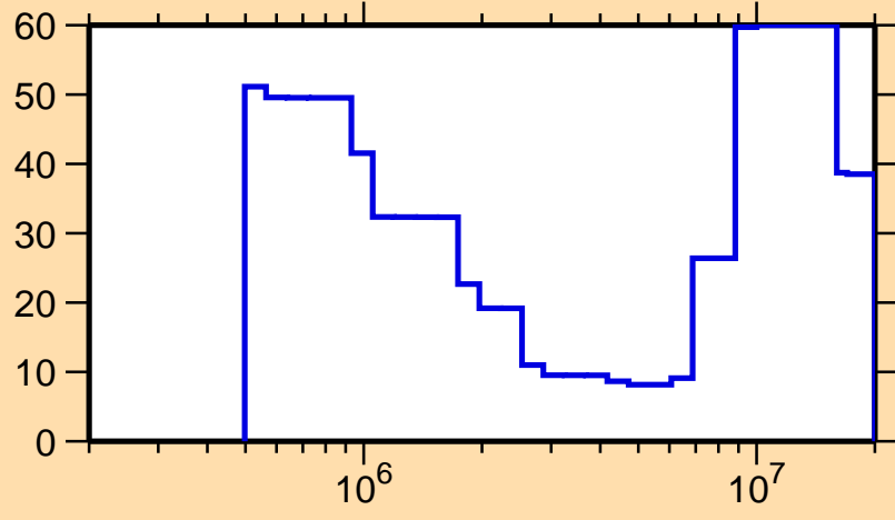
\Delta\sigma/\sigma vs. E for ^{157}\text{Dy}(n,n\text{cont.})
