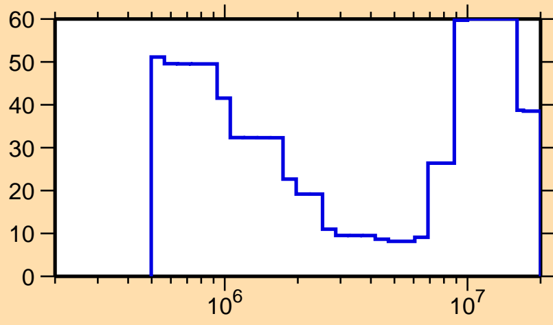
\Delta\sigma/\sigma vs. E for ^{157}\text{Dy}(n,n\text{cont.})
