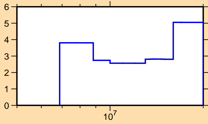
\Delta\sigma/\sigma vs. E for ^{157}\text{Dy}(n,\text{tot.})
