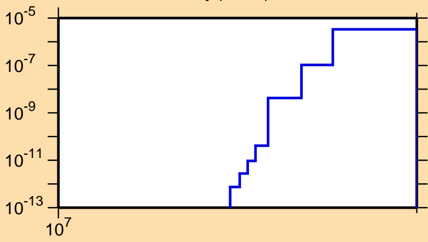
\sigma vs. E for ^{157}\text{Dy}(n,nd)
