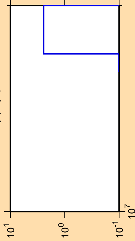
\Delta\sigma/\sigma vs. E for ^{157}\text{Dy}(n,pt)
