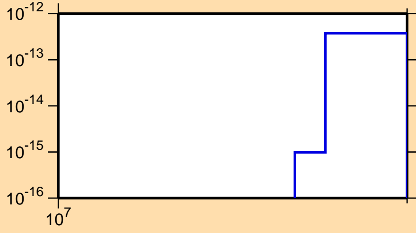
\sigma vs. E for ^{157}\text{Dy}(n,pd)
