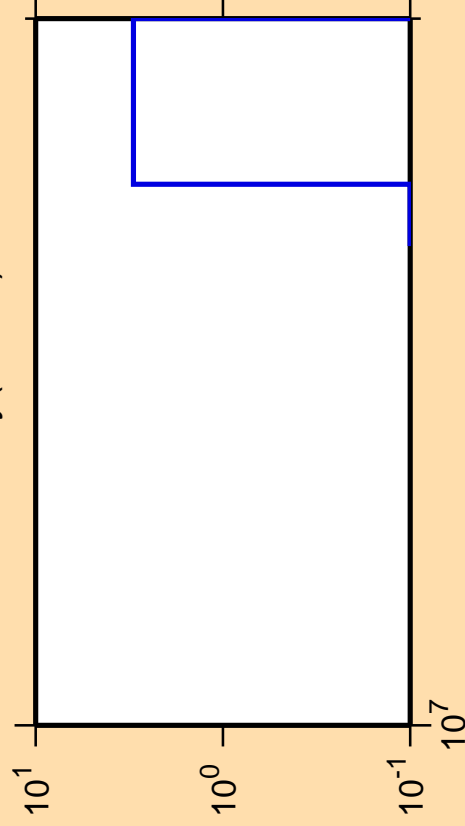
\Delta\sigma/\sigma vs. E for ^{157}\text{Dy} (mt 34)
