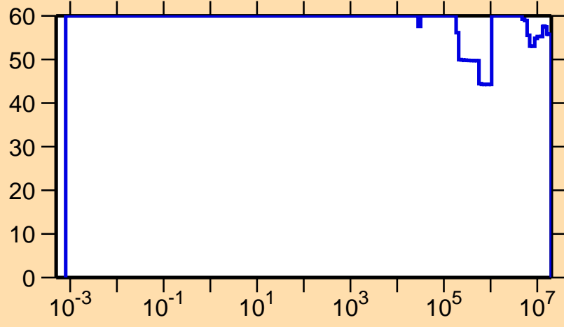
\Delta\sigma/\sigma vs. E for ^{157}\text{Dy}(n,p)
