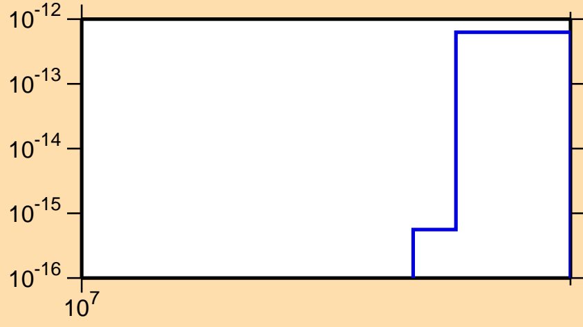
\sigma vs. E for ^{157}\text{Dy}(n,pt)
