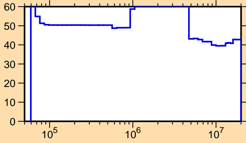
\Delta\sigma/\sigma vs. E for ^{157}\text{Dy}(n,n_1)
