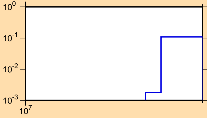
\sigma vs. E for ^{157}\text{Dy}(n,3n)
