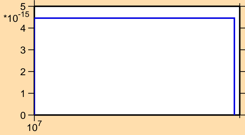
\sigma vs. E for ^{157}\text{Dy}(n,pt)
