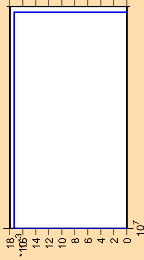
\Delta\sigma/\sigma vs. E for ^{157}\text{Dy}(n,pt)
