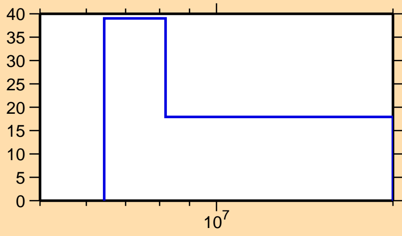
\Delta\sigma/\sigma vs. E for ^{157}\text{Dy}(n,2n)
