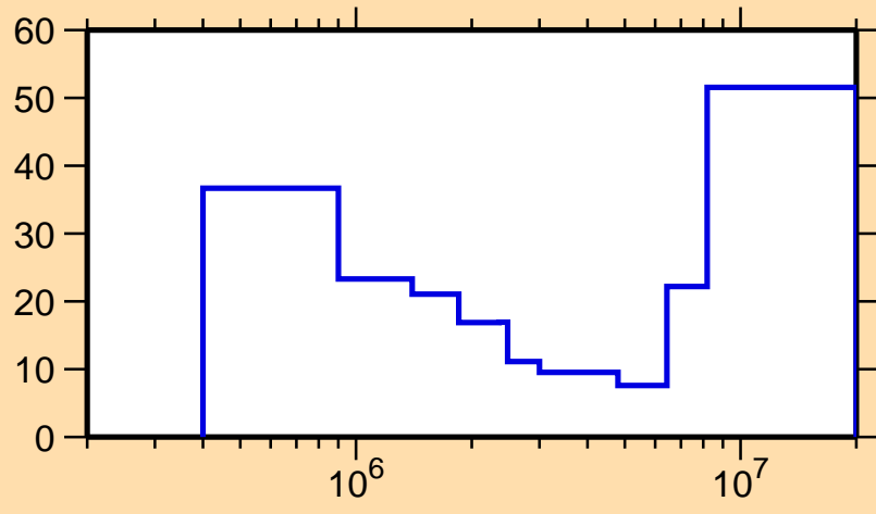
\Delta\sigma/\sigma vs. E for ^{157}\text{Dy}(n,inel.)
