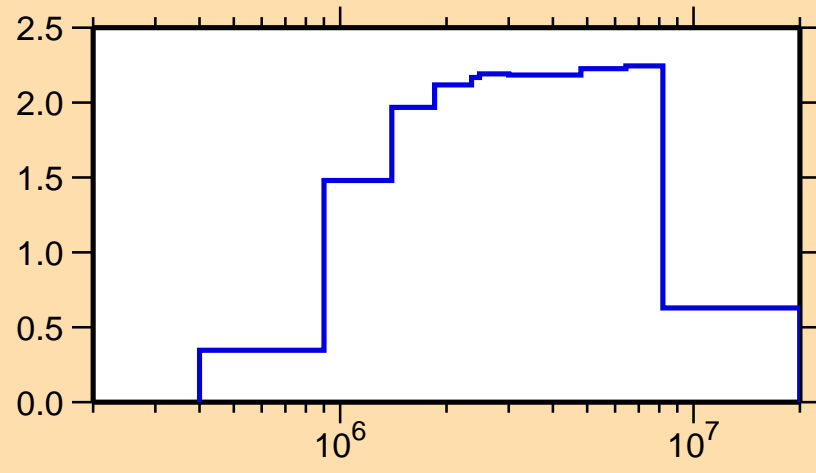
\sigma vs. E for ^{157}\text{Dy}(n,n\text{cont.})
