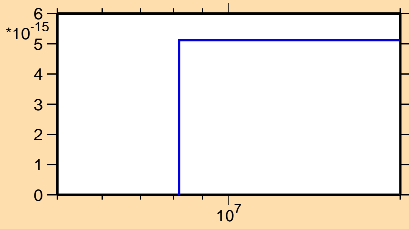
\sigma vs. E for ^{157}\text{Dy}(n,\text{pt})
