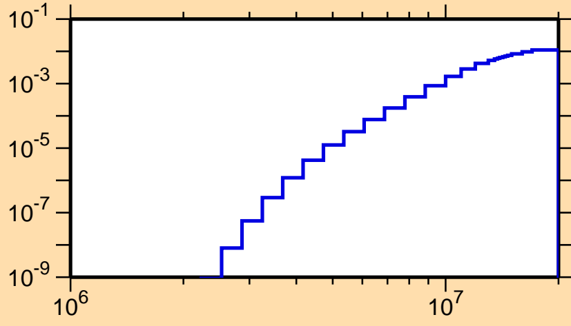
\sigma vs. E for ^{158}\text{Dy}(n,p)
