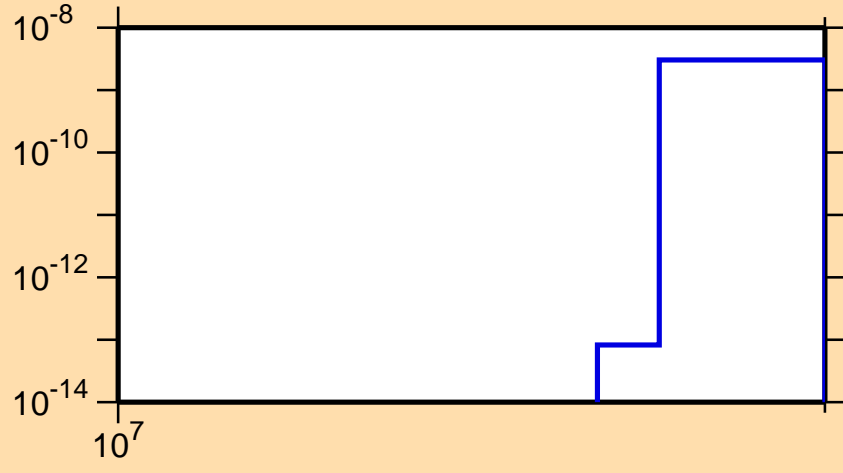
\sigma vs. E for ^{160}\text{Dy}(n,nt)
