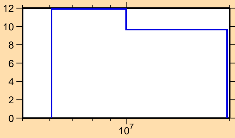
\Delta\sigma/\sigma vs. E for ^{160}\text{Dy}(n,2n)
