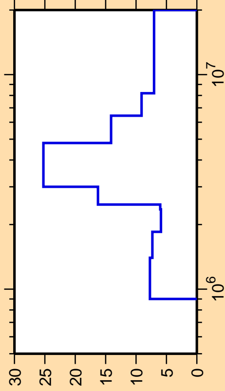
\Delta\sigma/\sigma vs. E for ^{160}\text{Dy}(n,n_4)
