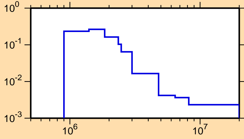
\sigma vs. E for ^{160}\text{Dy}(n,n_4)
