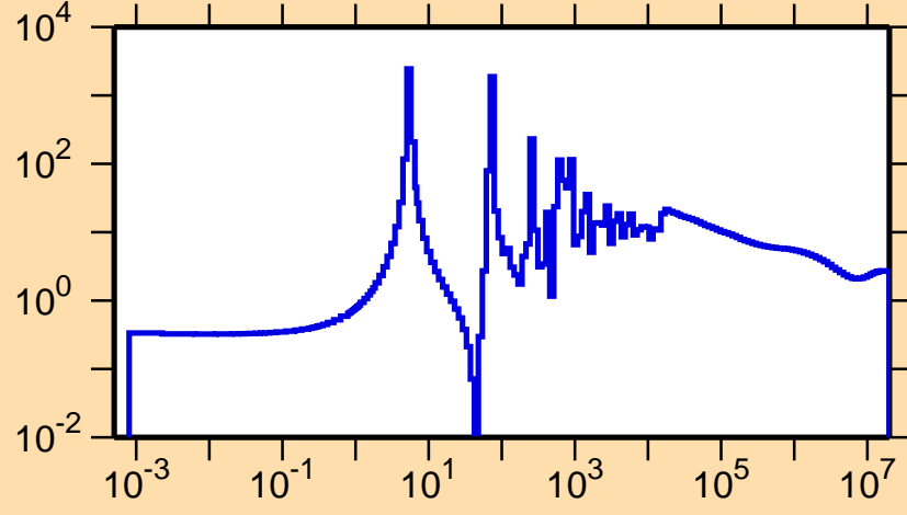
\sigma vs. E for ^{162}\text{Dy}(n,\text{el.})
