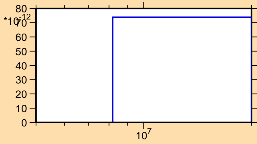
\sigma vs. E for ^{162}\text{Dy}(n,nt)
