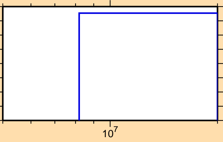
\sigma vs. E for ^{165}\text{Dy}(n,t)
