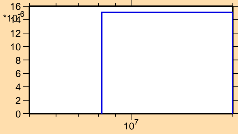
\sigma vs. E for ^{165}\text{Dy}(n,t)
