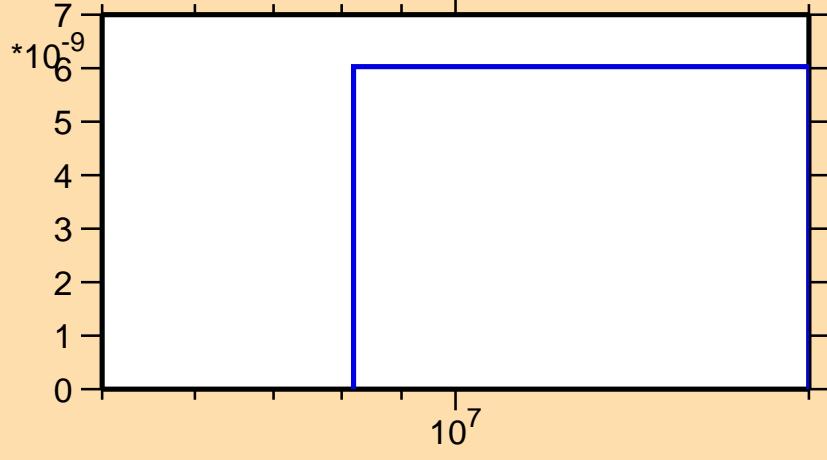
\sigma vs. E for ^{165}\text{Dy}(n,nd)
