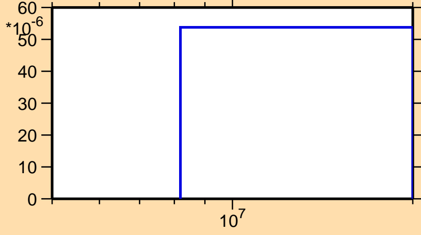
\sigma vs. E for ^{165}\text{Dy}(n,np)
