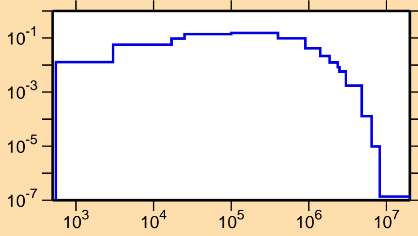
\sigma vs. E for ^{165}\text{Dy}(n,n_1)
