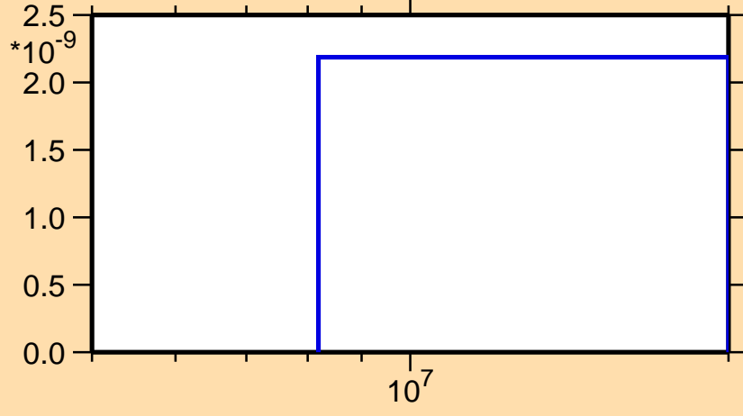
\sigma vs. E for ^{165}\text{Dy}(n,2n\alpha)
