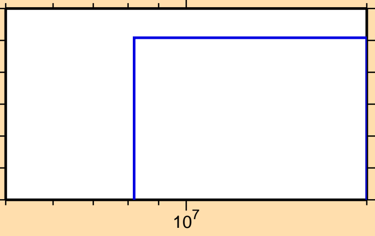
\sigma vs. E for ^{165}\text{Dy}(n,nd)
