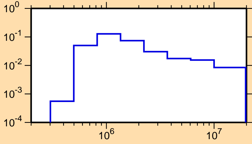
\sigma vs. E for ^{167}\text{Dy}(n,n_4)
