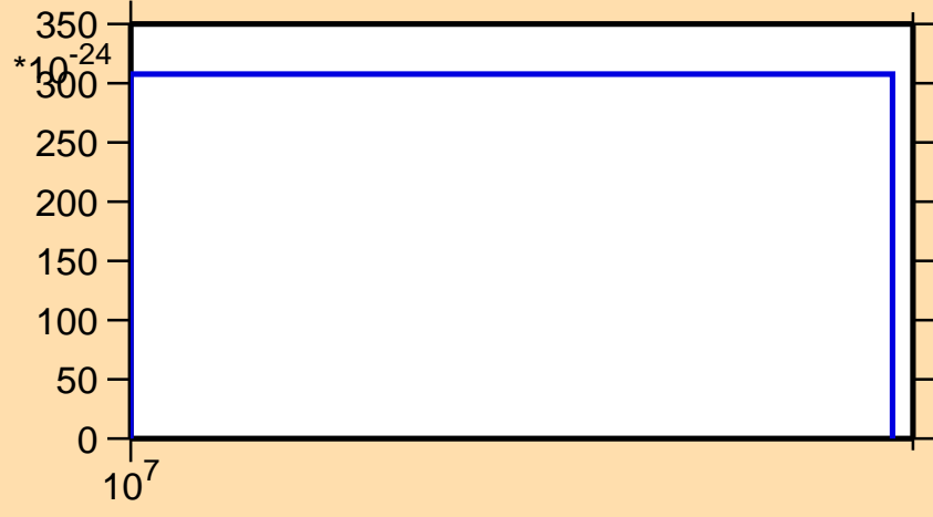
\sigma vs. E for ^{167}\text{Dy} (mt 11)
