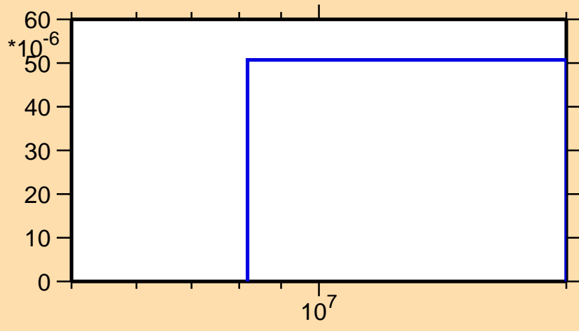
\sigma vs. E for ^{167}\text{Dy}(n,d)
