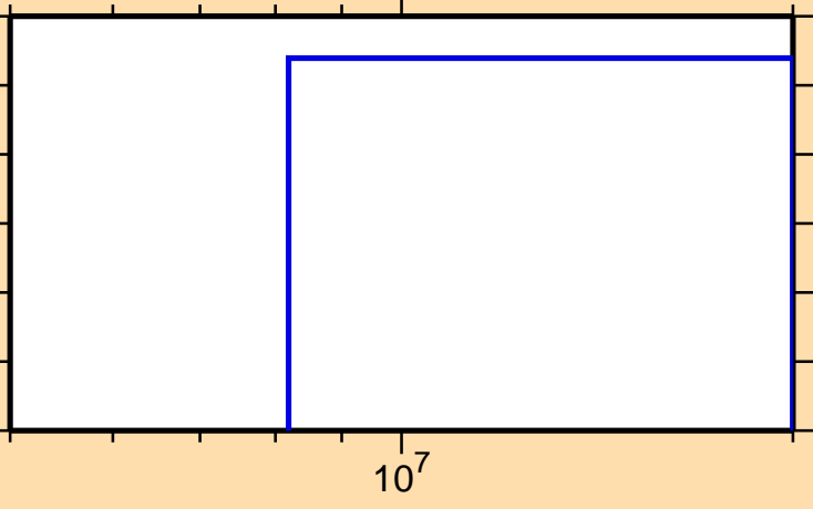
\sigma vs. E for ^{167}\text{Dy}(n,n\alpha)
