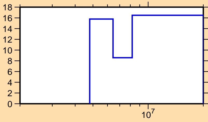
\Delta\sigma/\sigma vs. E for ^{167}\text{Dy}(n,2n)
